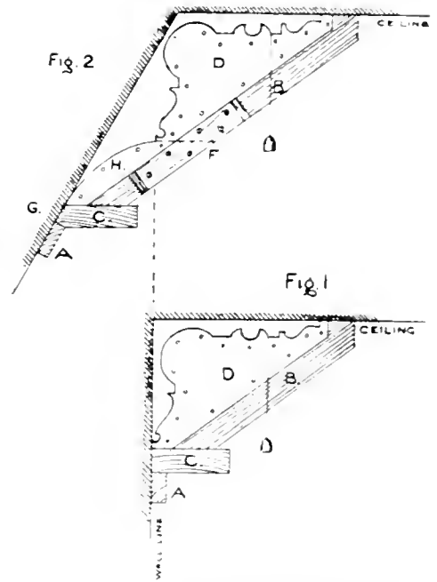
NO. 125. RUNNING MOULD FOR SQUARE AND SPLOYED ANGLES.
